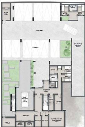
BASEMENT 9,195 SQ.FT
